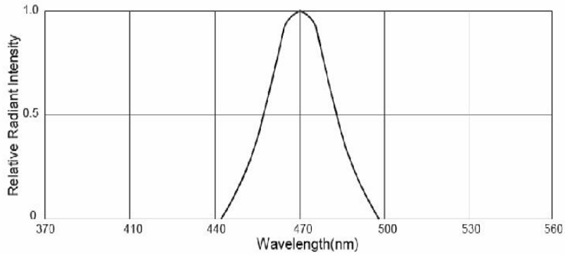
Fig.1 Relative Radiant Intensity VS. Wavelength
